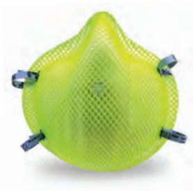
▲ 2200HVN95
