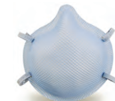
● 2212GN95-M/L
