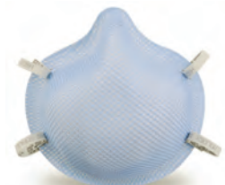
● 2211GN95-S
