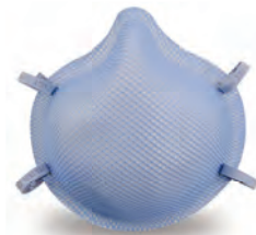
● 1512 N95 M
