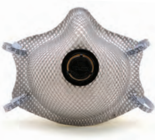
● 2400N95
