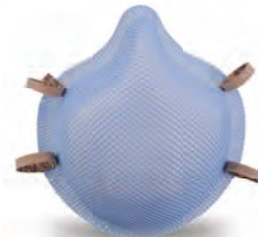
● 1513 N95 G
