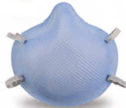
● 1511 N95 P
