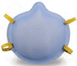
● 1510 N95 XP
