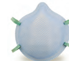
● 2217GN95-LP
